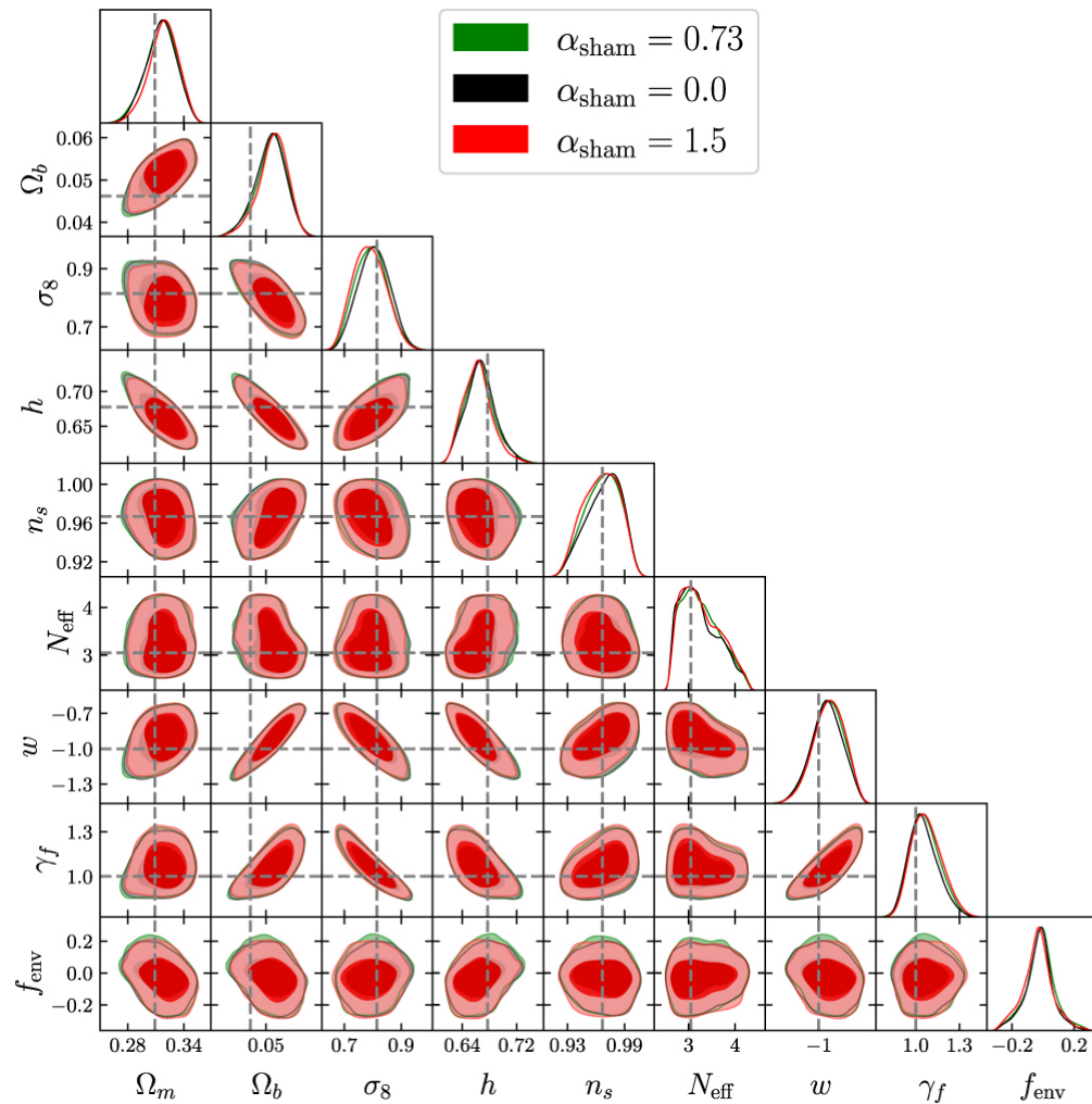
Figure 19. from Zhongxu Zhai et al 2023 Astrophys. J. 948 doi:10.3847/1538-4357/acc65b https://dx.doi.org/10.3847/1538-4357/acc65b © 2023. The Author(s). Published by the American Astronomical Society.
