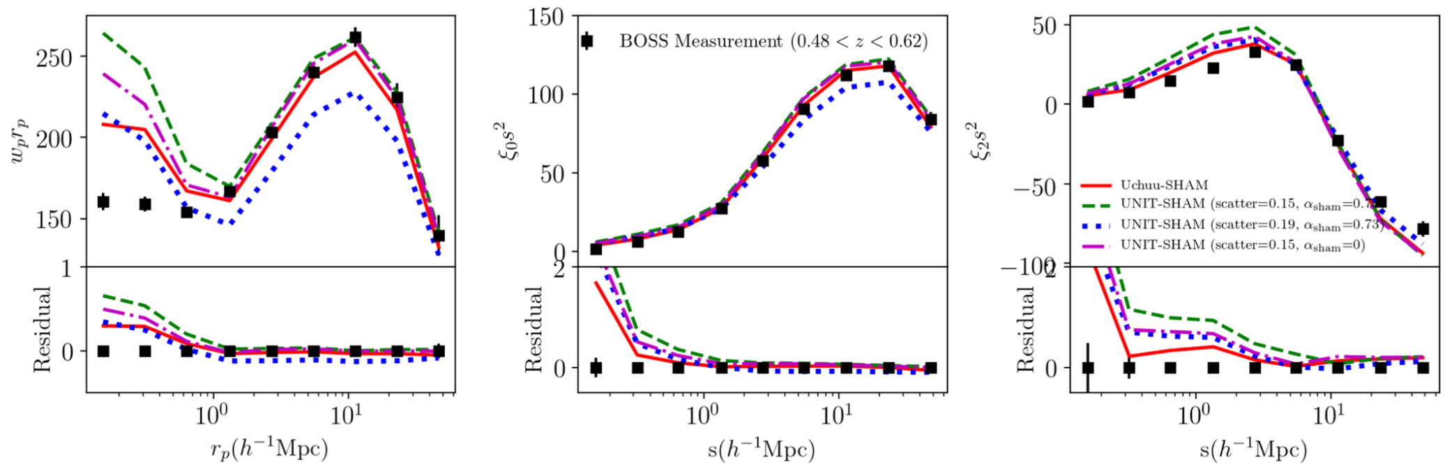
Figure 17. from Zhongxu Zhai et al 2023 Astrophys. J. 948 doi:10.3847/1538-4357/acc65b https://dx.doi.org/10.3847/1538-4357/acc65b © 2023. The Author(s). Published by the American Astronomical Society.
