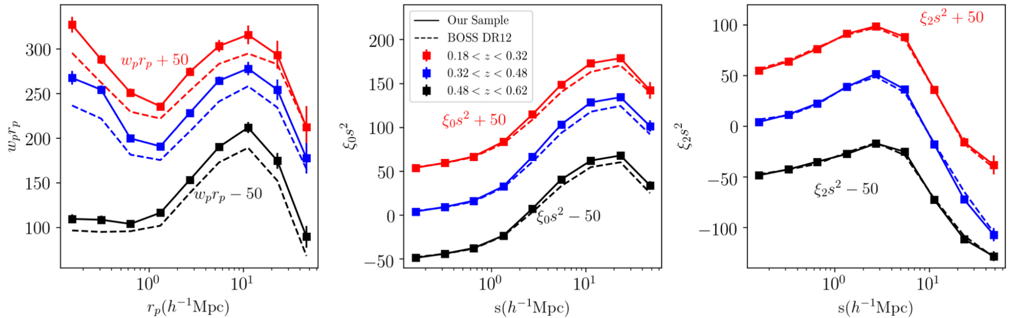
Figure 12. from Zhongxu Zhai et al 2023 Astrophys. J. 948 doi:10.3847/1538-4357/acc65b https://dx.doi.org/10.3847/1538-4357/acc65b © 2023. The Author(s). Published by the American Astronomical Society.
