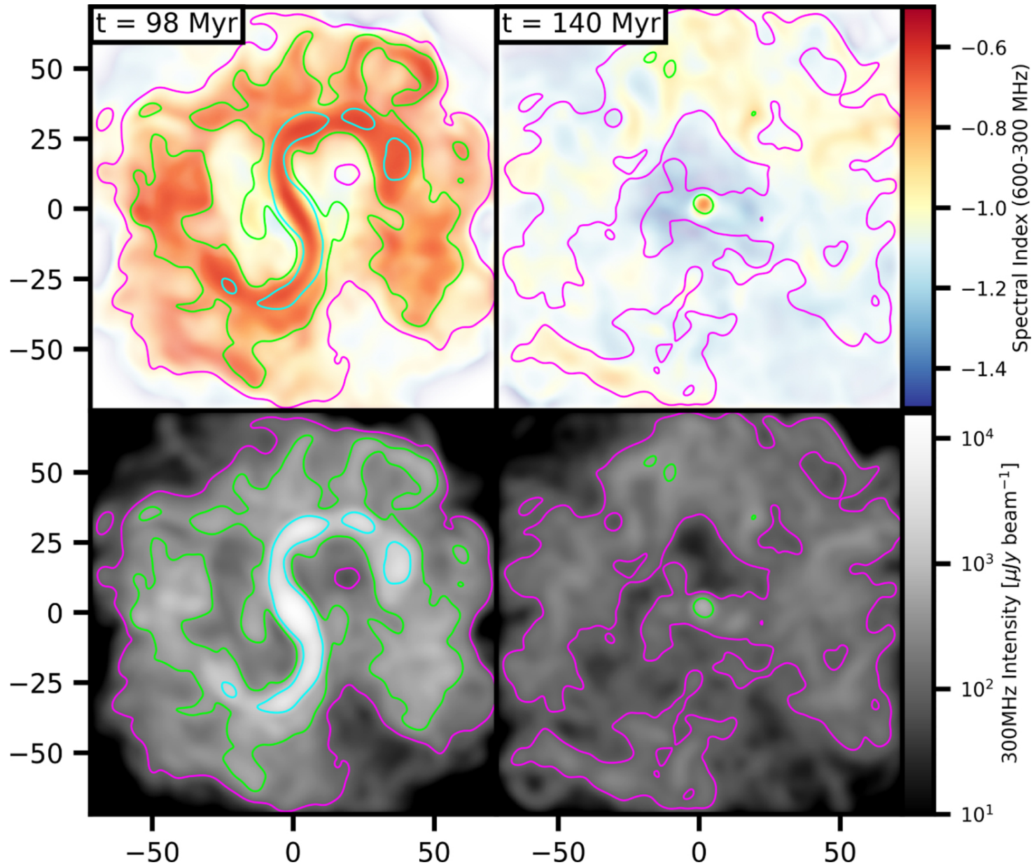
Figure 5. from Chris Nolting et al 2023 Astrophys. J. 948 doi:10.3847/1538-4357/acc652 https://dx.doi.org/10.3847/1538-4357/acc652 © 2023. The Author(s). Published by the American Astronomical Society.
