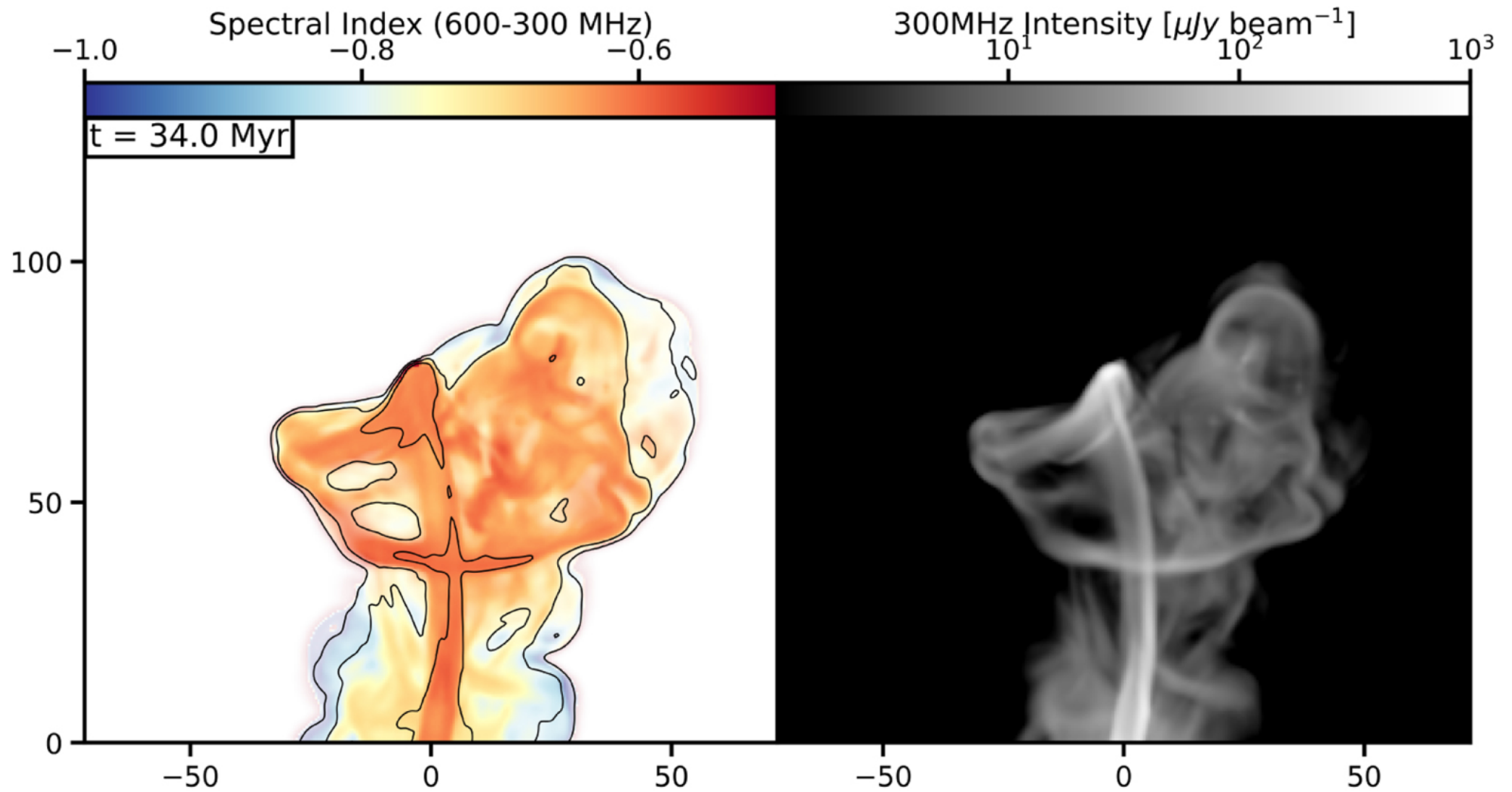
Figure 4. from Chris Nolting et al 2023 Astrophys. J. 948 doi:10.3847/1538-4357/acc652 https://dx.doi.org/10.3847/1538-4357/acc652 © 2023. The Author(s). Published by the American Astronomical Society.
