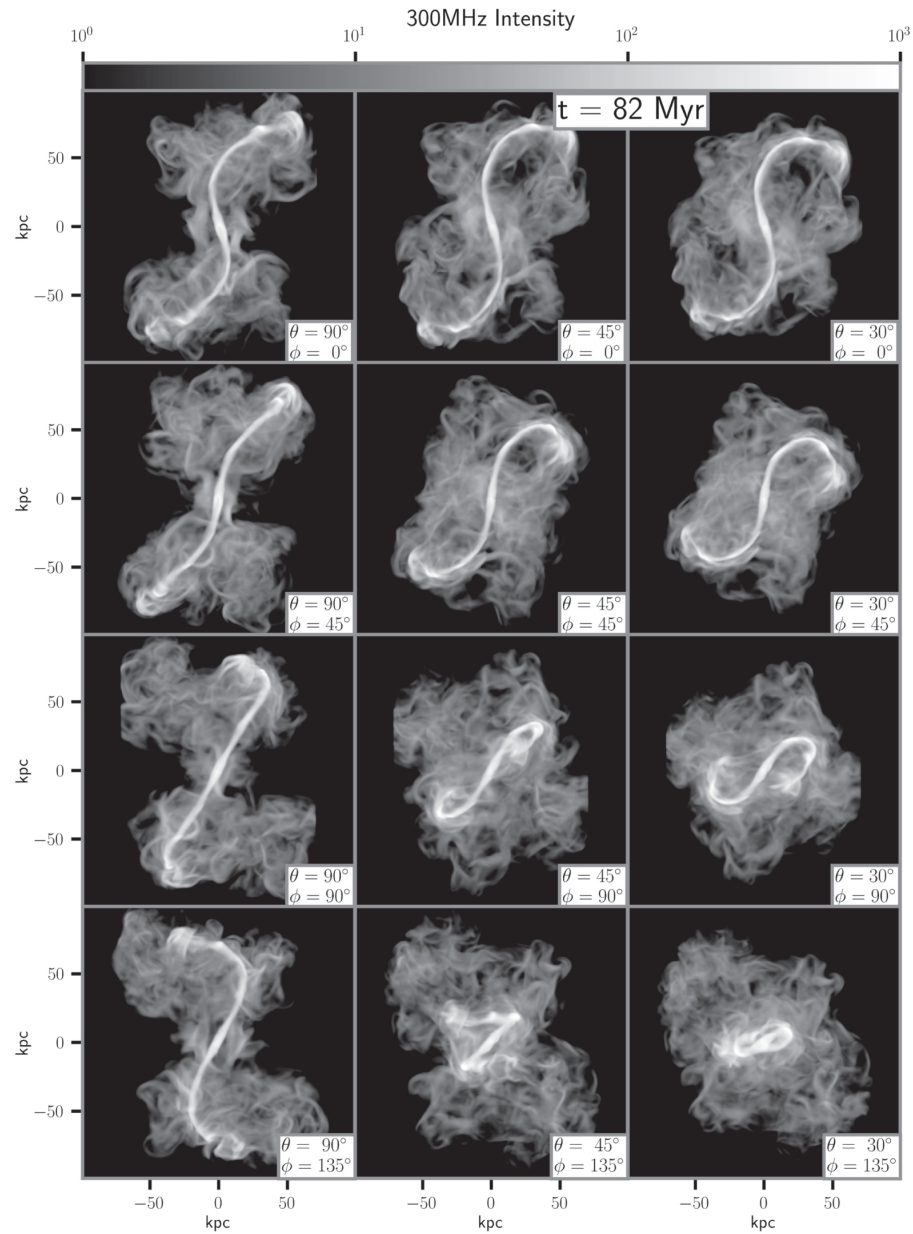
Figure 3. from Chris Nolting et al 2023 Astrophys. J. 948 doi:10.3847/1538-4357/acc652 https://dx.doi.org/10.3847/1538-4357/acc652 © 2023. The Author(s). Published by the American Astronomical Society.
