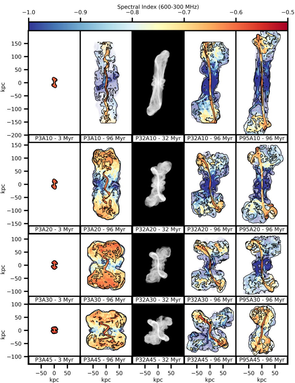
Figure 2. from Chris Nolting et al 2023 Astrophys. J. 948 doi:10.3847/1538-4357/acc652 https://dx.doi.org/10.3847/1538-4357/acc652 © 2023. The Author(s). Published by the American Astronomical Society.
