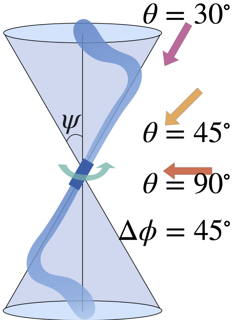
Figure 1. from Chris Nolting et al 2023 Astrophys. J. 948 doi:10.3847/1538-4357/acc652 https://dx.doi.org/10.3847/1538-4357/acc652 © 2023. The Author(s). Published by the American Astronomical Society.
