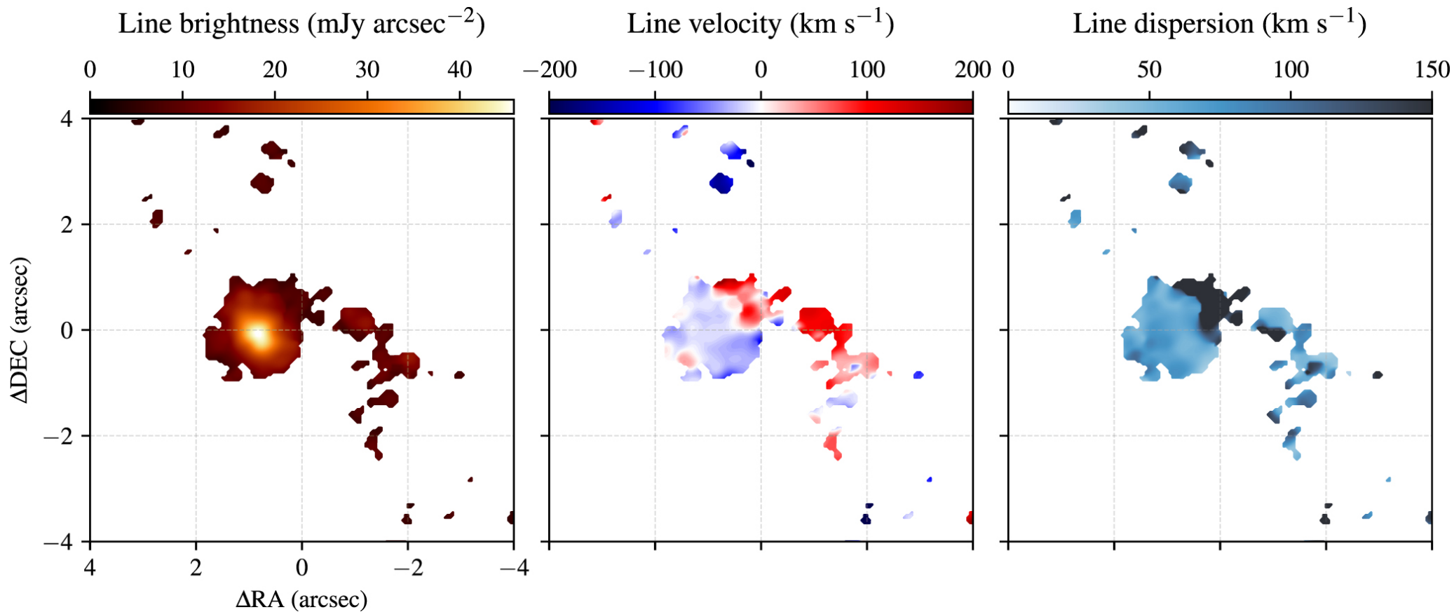
Figure 8. from Dominic W. Pesce et al 2023 Astrophys. J. 948 doi:10.3847/1538-4357/acc57a https://dx.doi.org/10.3847/1538-4357/acc57a © 2023. The Author(s). Published by the American Astronomical Society.
