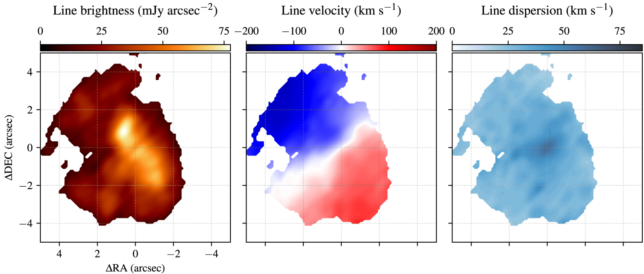
Figure 6. from Dominic W. Pesce et al 2023 Astrophys. J. 948 doi:10.3847/1538-4357/acc57a https://dx.doi.org/10.3847/1538-4357/acc57a © 2023. The Author(s). Published by the American Astronomical Society.
