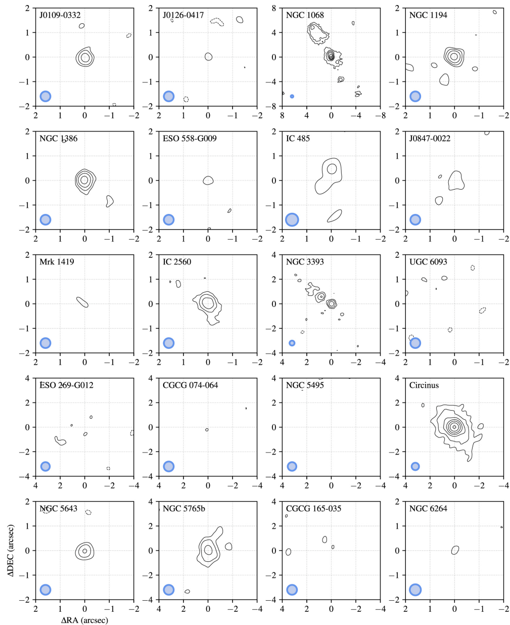
Figure 5. from Dominic W. Pesce et al 2023 Astrophys. J. 948 doi:10.3847/1538-4357/acc57a https://dx.doi.org/10.3847/1538-4357/acc57a © 2023. The Author(s). Published by the American Astronomical Society.
