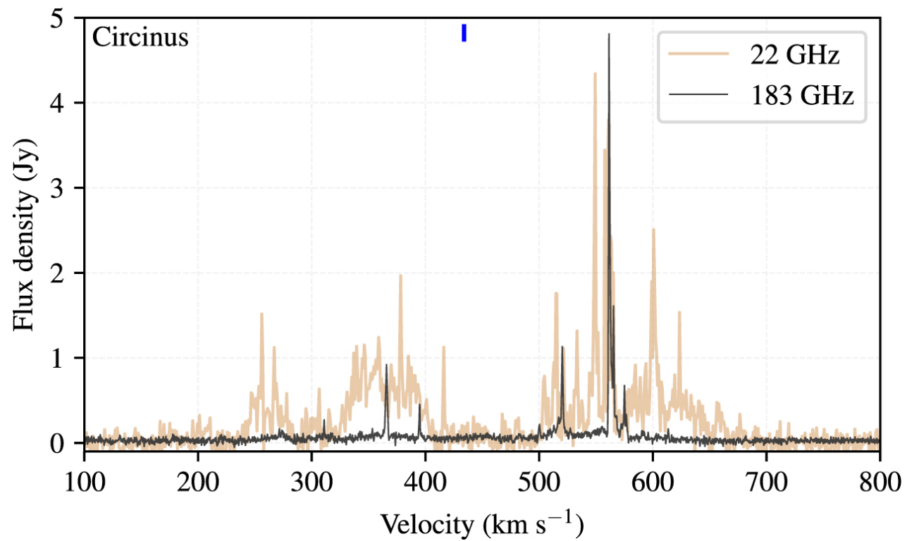
Figure 3. from Dominic W. Pesce et al 2023 Astrophys. J. 948 doi:10.3847/1538-4357/acc57a https://dx.doi.org/10.3847/1538-4357/acc57a © 2023. The Author(s). Published by the American Astronomical Society.
