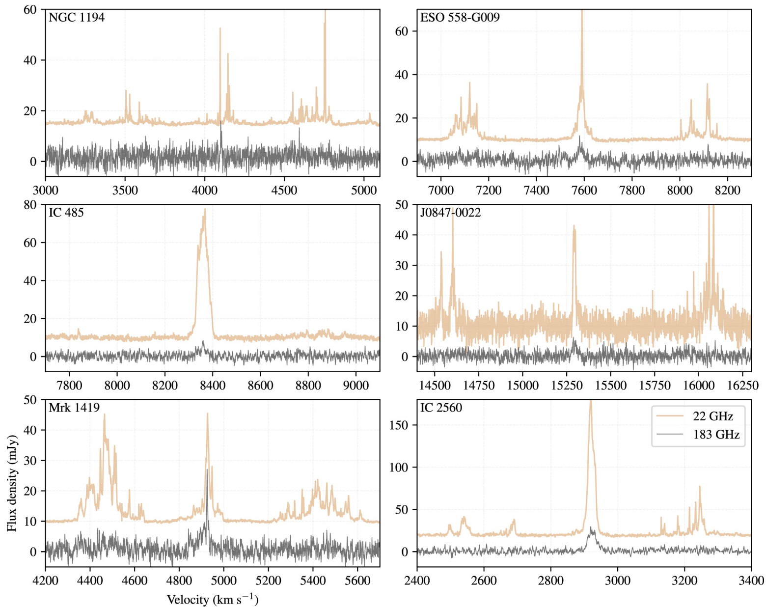
Figure 1. from Dominic W. Pesce et al 2023 Astrophys. J. 948 doi:10.3847/1538-4357/acc57a https://dx.doi.org/10.3847/1538-4357/acc57a © 2023. The Author(s). Published by the American Astronomical Society.
