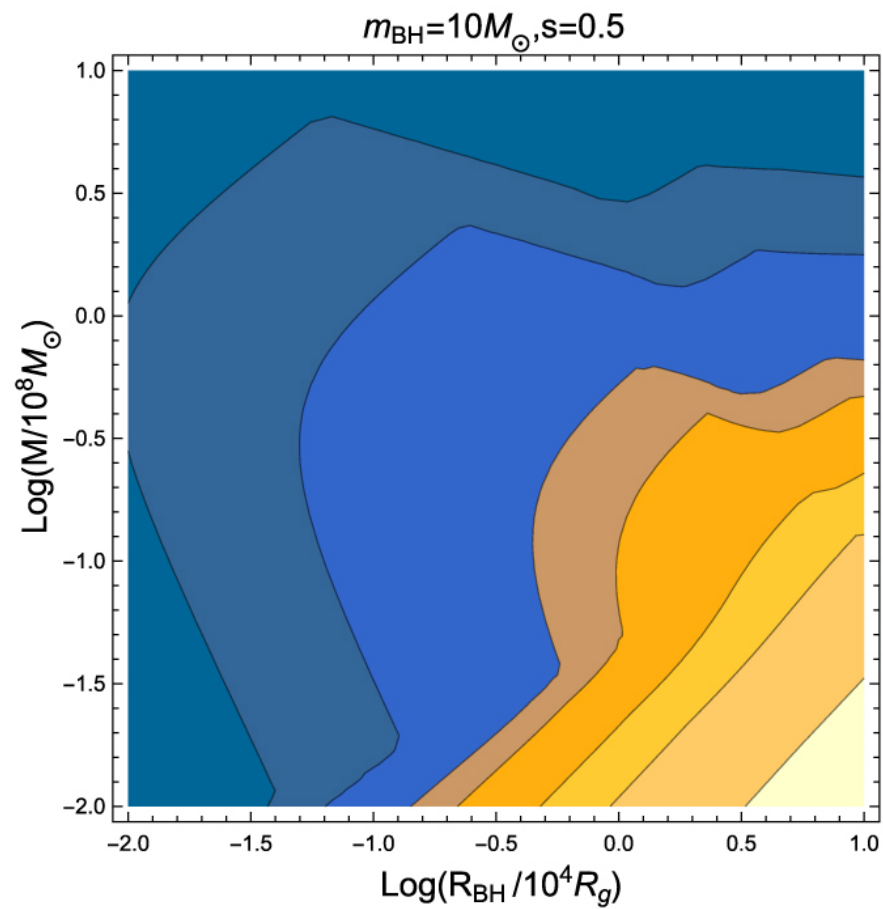
Figure 9. from Ken Chen et al 2023 Astrophys. J. 948 doi:10.3847/1538-4357/acc45f https://dx.doi.org/10.3847/1538-4357/acc45f © 2023. The Author(s). Published by the American Astronomical Society.
