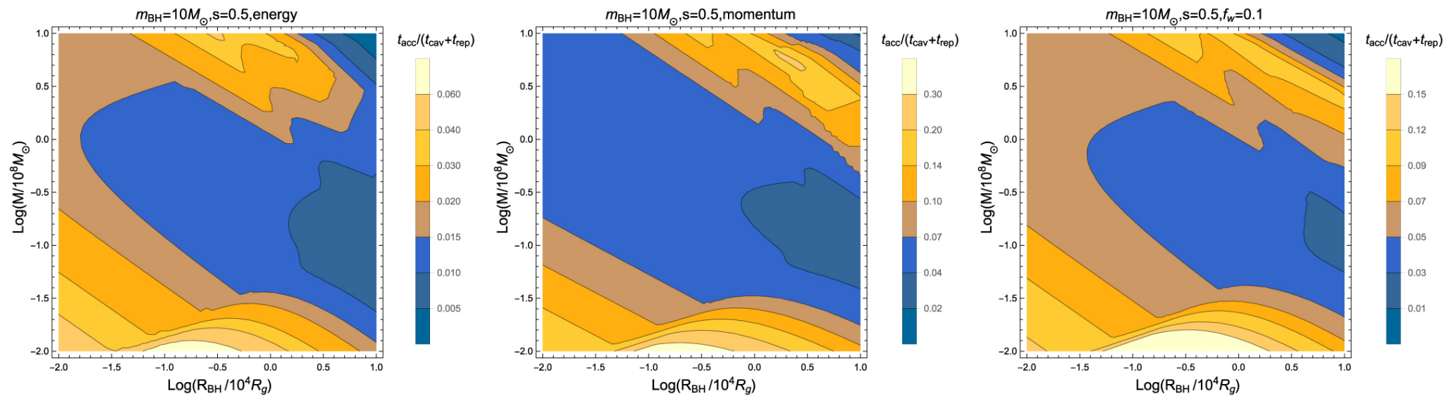
Figure 8. from Ken Chen et al 2023 Astrophys. J. 948 doi:10.3847/1538-4357/acc45f https://dx.doi.org/10.3847/1538-4357/acc45f © 2023. The Author(s). Published by the American Astronomical Society.
