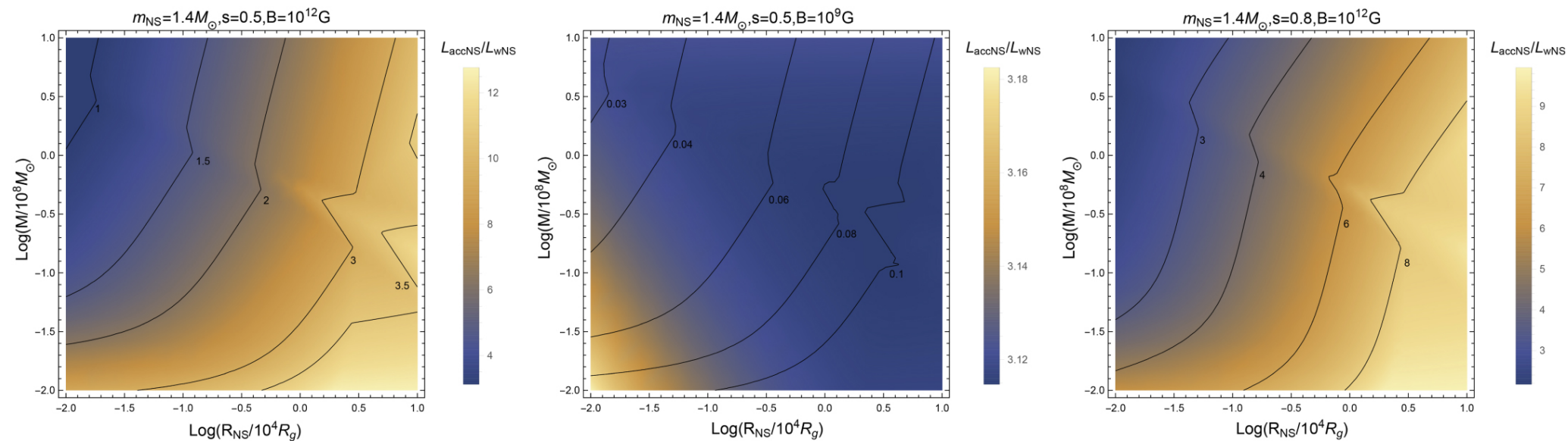
Figure 6. from Ken Chen et al 2023 Astrophys. J. 948 doi:10.3847/1538-4357/acc45f https://dx.doi.org/10.3847/1538-4357/acc45f © 2023. The Author(s). Published by the American Astronomical Society.
