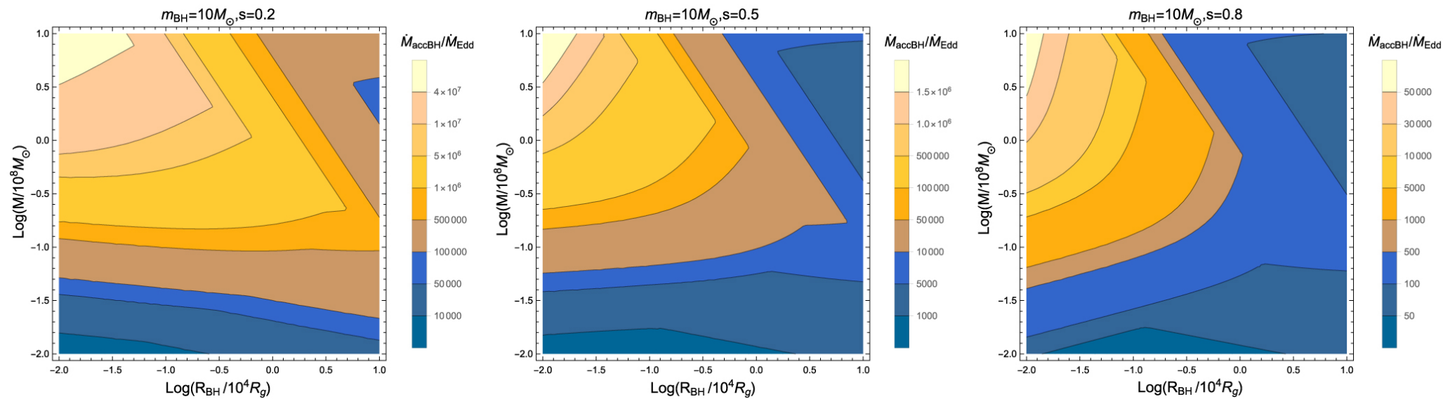
Figure 2. from Ken Chen et al 2023 Astrophys. J. 948 doi:10.3847/1538-4357/acc45f https://dx.doi.org/10.3847/1538-4357/acc45f © 2023. The Author(s). Published by the American Astronomical Society.
