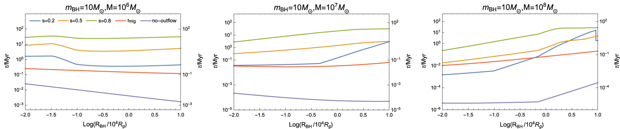
Figure 13. from Ken Chen et al 2023 Astrophys. J. 948 doi:10.3847/1538-4357/acc45f https://dx.doi.org/10.3847/1538-4357/acc45f © 2023. The Author(s). Published by the American Astronomical Society.
