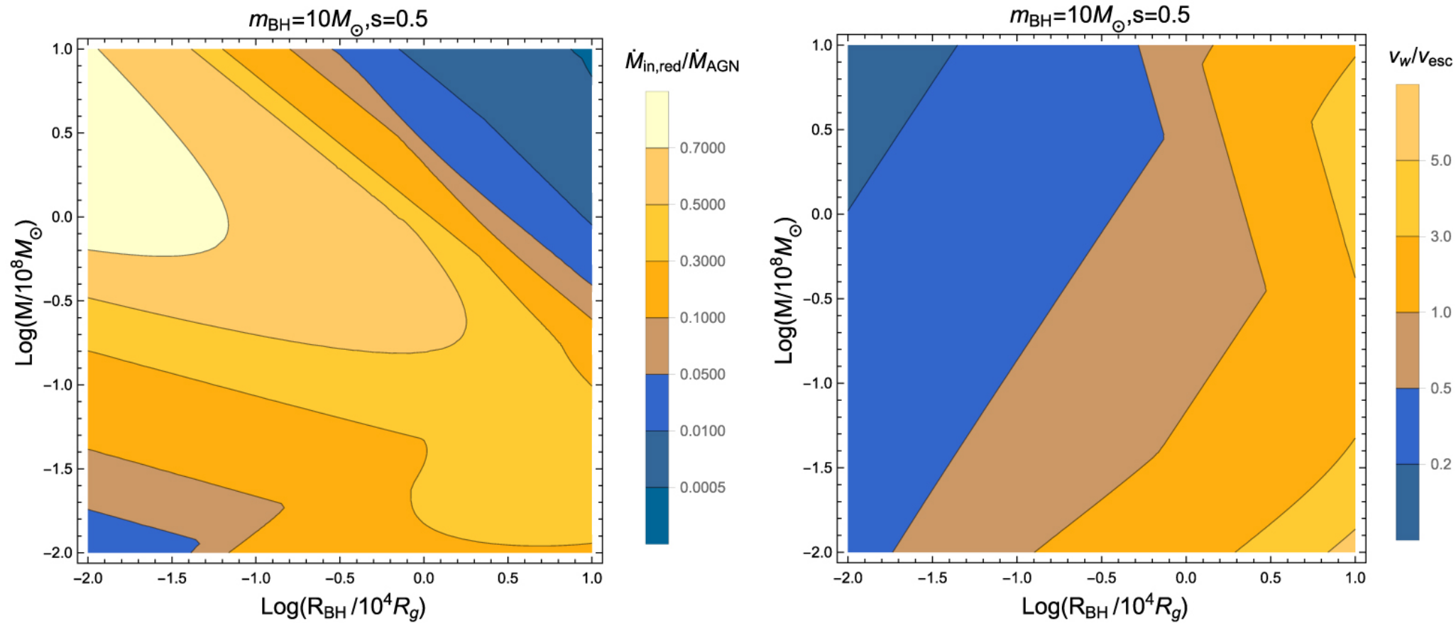
Figure 11. from Ken Chen et al 2023 Astrophys. J. 948 doi:10.3847/1538-4357/acc45f https://dx.doi.org/10.3847/1538-4357/acc45f © 2023. The Author(s). Published by the American Astronomical Society.
