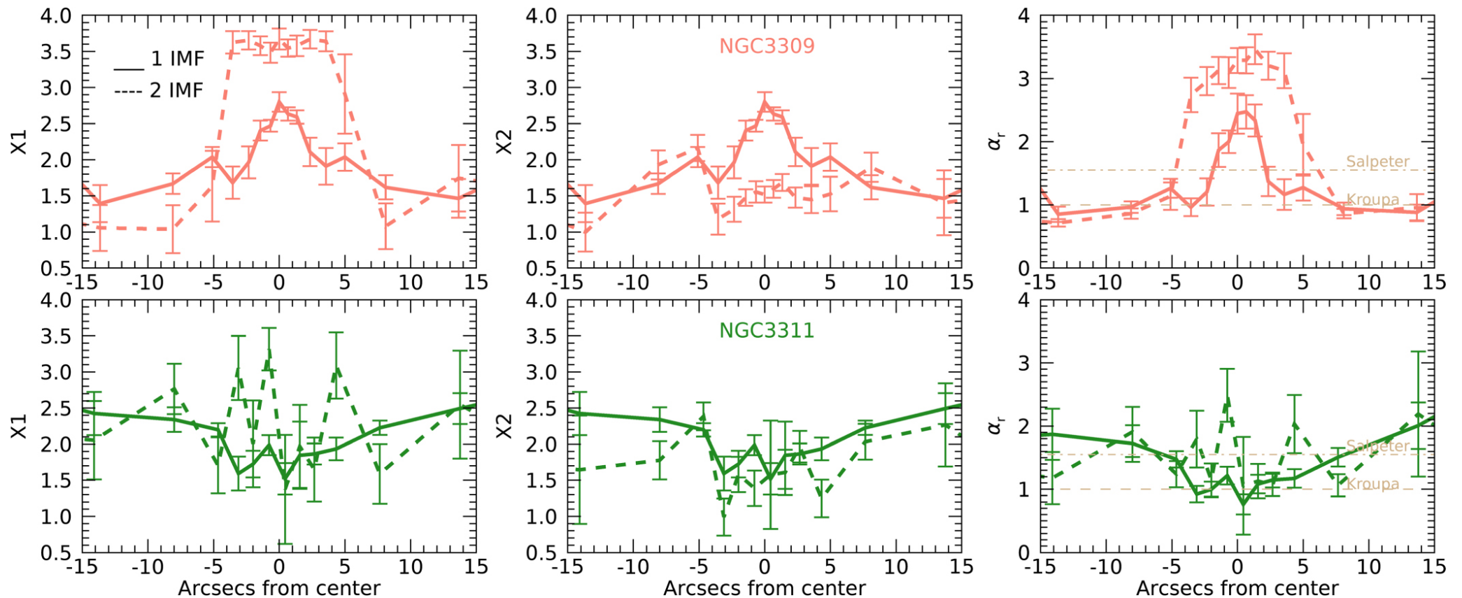
Figure 8. from Ilaria Lonoce et al 2023 Astrophys. J. 948 doi:10.3847/1538-4357/acc025 https://dx.doi.org/10.3847/1538-4357/acc025 © 2023. The Author(s). Published by the American Astronomical Society.
