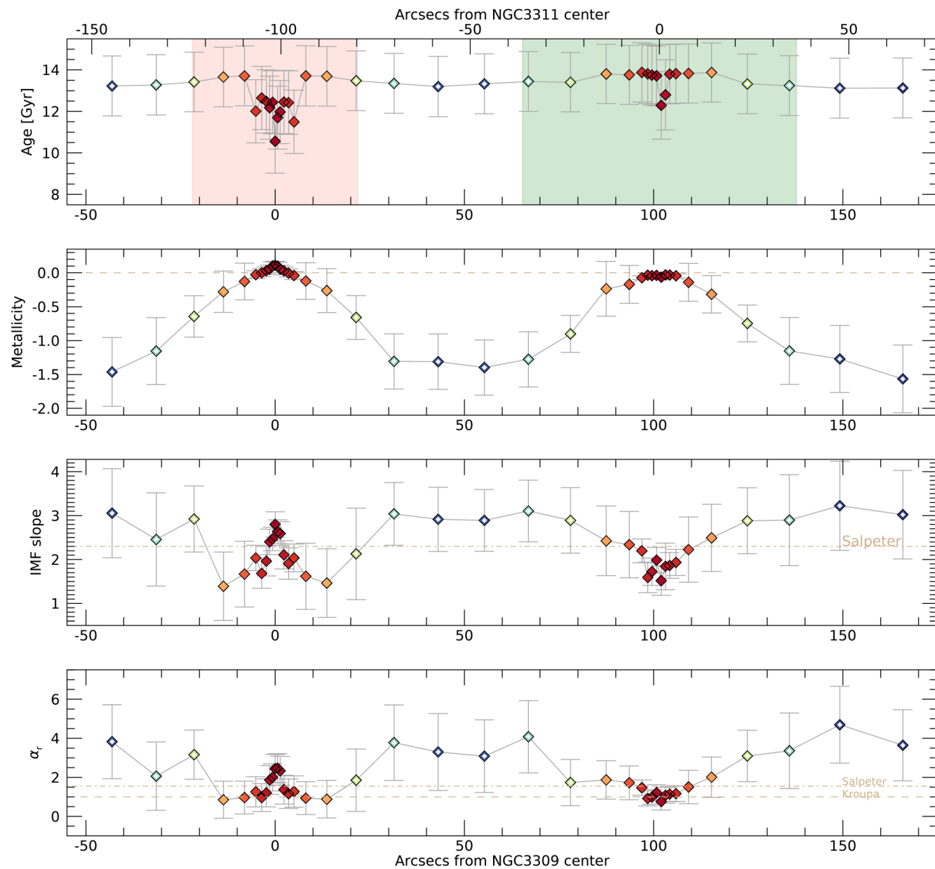
Figure 6. from Ilaria Lonoce et al 2023 Astrophys. J. 948 doi:10.3847/1538-4357/acc025 https://dx.doi.org/10.3847/1538-4357/acc025 © 2023. The Author(s). Published by the American Astronomical Society.
