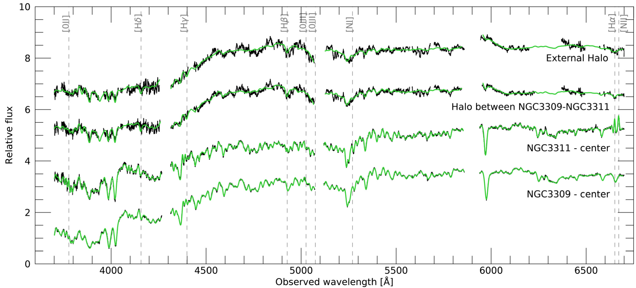
Figure 5. from Ilaria Lonoce et al 2023 Astrophys. J. 948 doi:10.3847/1538-4357/acc025 https://dx.doi.org/10.3847/1538-4357/acc025 © 2023. The Author(s). Published by the American Astronomical Society.
