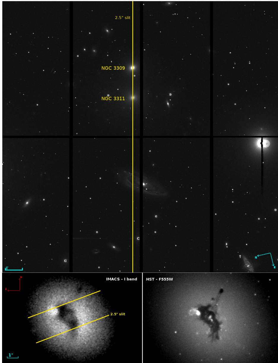
Figure 4. from Ilaria Lonoce et al 2023 Astrophys. J. 948 doi:10.3847/1538-4357/acc025 https://dx.doi.org/10.3847/1538-4357/acc025 © 2023. The Author(s). Published by the American Astronomical Society.
