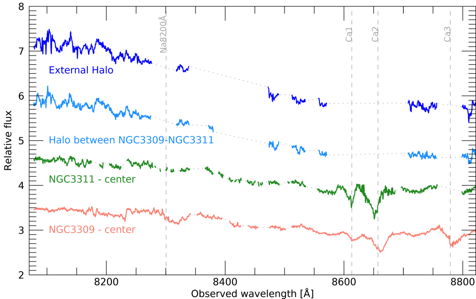
Figure 3. from Ilaria Lonoce et al 2023 Astrophys. J. 948 doi:10.3847/1538-4357/acc025 https://dx.doi.org/10.3847/1538-4357/acc025 © 2023. The Author(s). Published by the American Astronomical Society.
