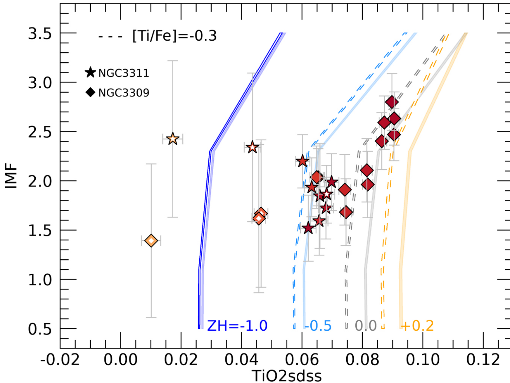
Figure 17. from Ilaria Lonoce et al 2023 Astrophys. J. 948 doi:10.3847/1538-4357/acc025 https://dx.doi.org/10.3847/1538-4357/acc025 © 2023. The Author(s). Published by the American Astronomical Society.
