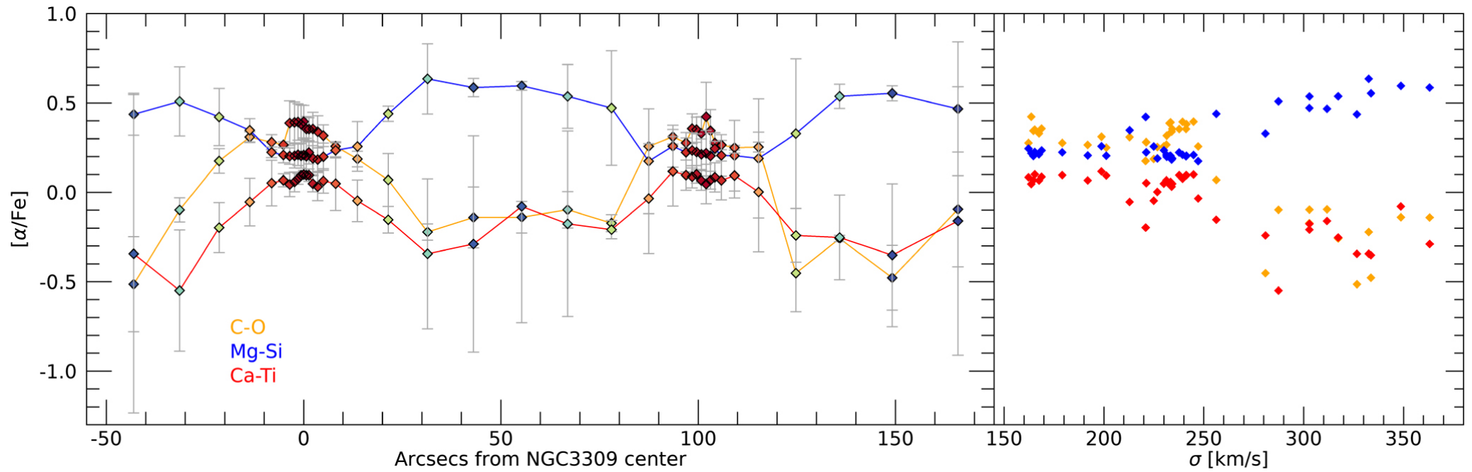
Figure 14. from Ilaria Lonoce et al 2023 Astrophys. J. 948 doi:10.3847/1538-4357/acc025 https://dx.doi.org/10.3847/1538-4357/acc025 © 2023. The Author(s). Published by the American Astronomical Society.
