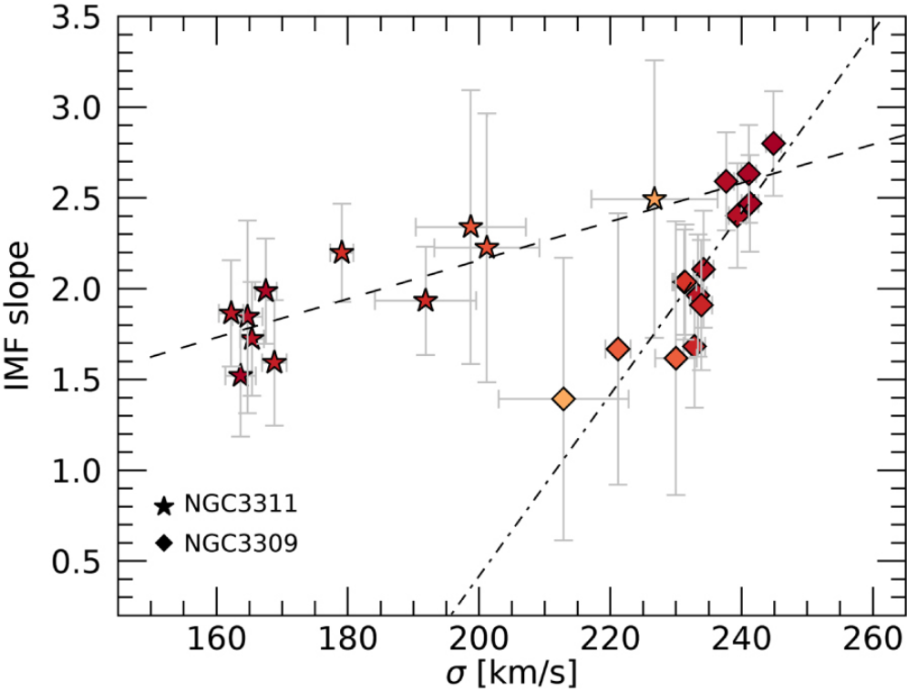
Figure 11. from Ilaria Lonoce et al 2023 Astrophys. J. 948 doi:10.3847/1538-4357/acc025 https://dx.doi.org/10.3847/1538-4357/acc025 © 2023. The Author(s). Published by the American Astronomical Society.
