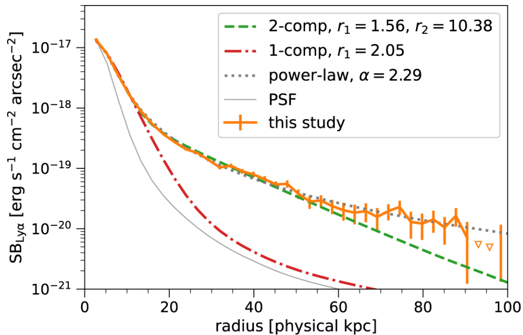
Figure 9. from Satoshi Kikuta et al 2023 Astrophys. J. 947 doi:10.3847/1538-4357/acbf30 https://dx.doi.org/10.3847/1538-4357/acbf30 © 2023. The Author(s). Published by the American Astronomical Society.
