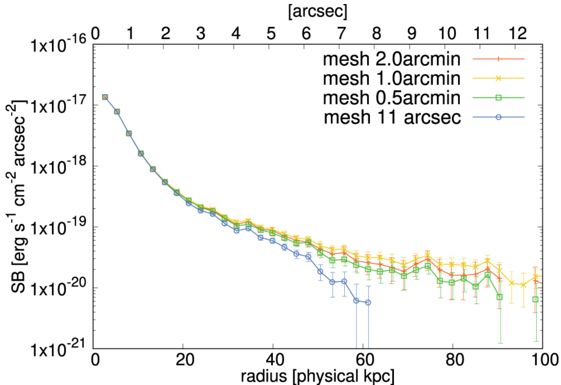
Figure 8. from Satoshi Kikuta et al 2023 Astrophys. J. 947 doi:10.3847/1538-4357/acbf30 https://dx.doi.org/10.3847/1538-4357/acbf30 © 2023. The Author(s). Published by the American Astronomical Society.
