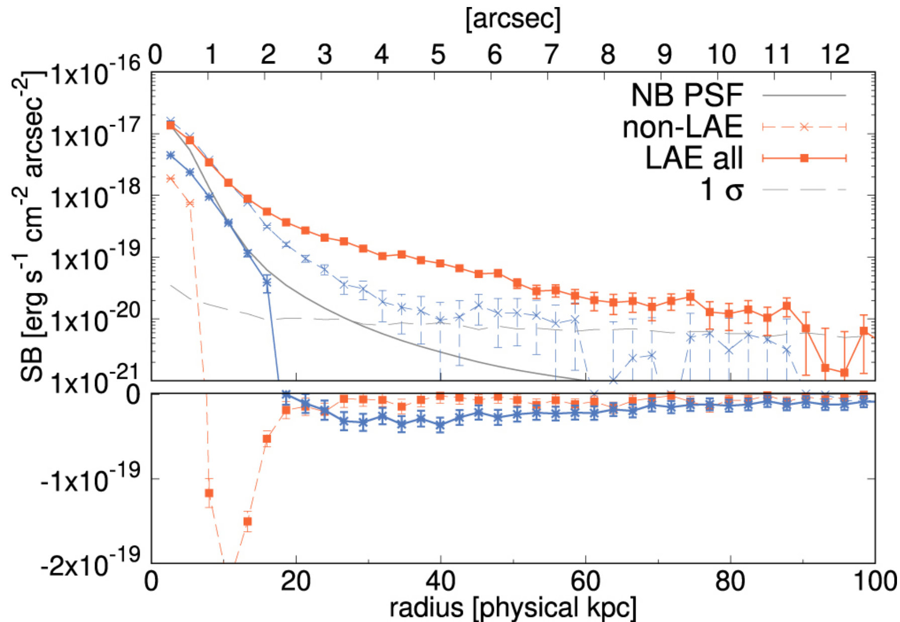
Figure 7. from Satoshi Kikuta et al 2023 Astrophys. J. 947 doi:10.3847/1538-4357/acbf30 https://dx.doi.org/10.3847/1538-4357/acbf30 © 2023. The Author(s). Published by the American Astronomical Society.
