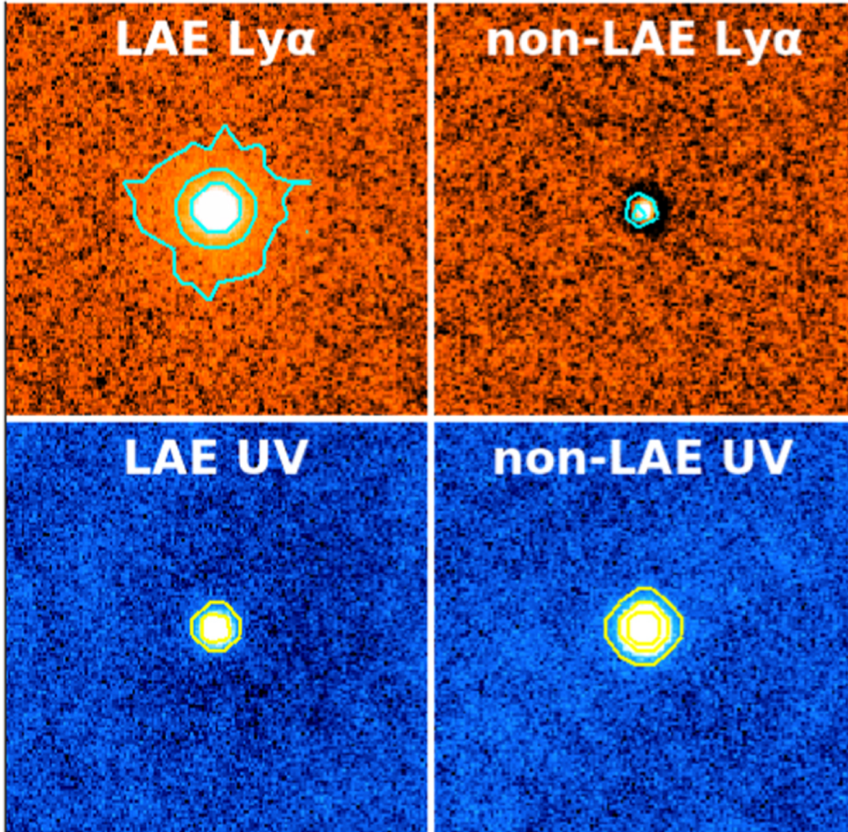
Figure 6. from Satoshi Kikuta et al 2023 Astrophys. J. 947 doi:10.3847/1538-4357/acbf30 https://dx.doi.org/10.3847/1538-4357/acbf30 © 2023. The Author(s). Published by the American Astronomical Society.
