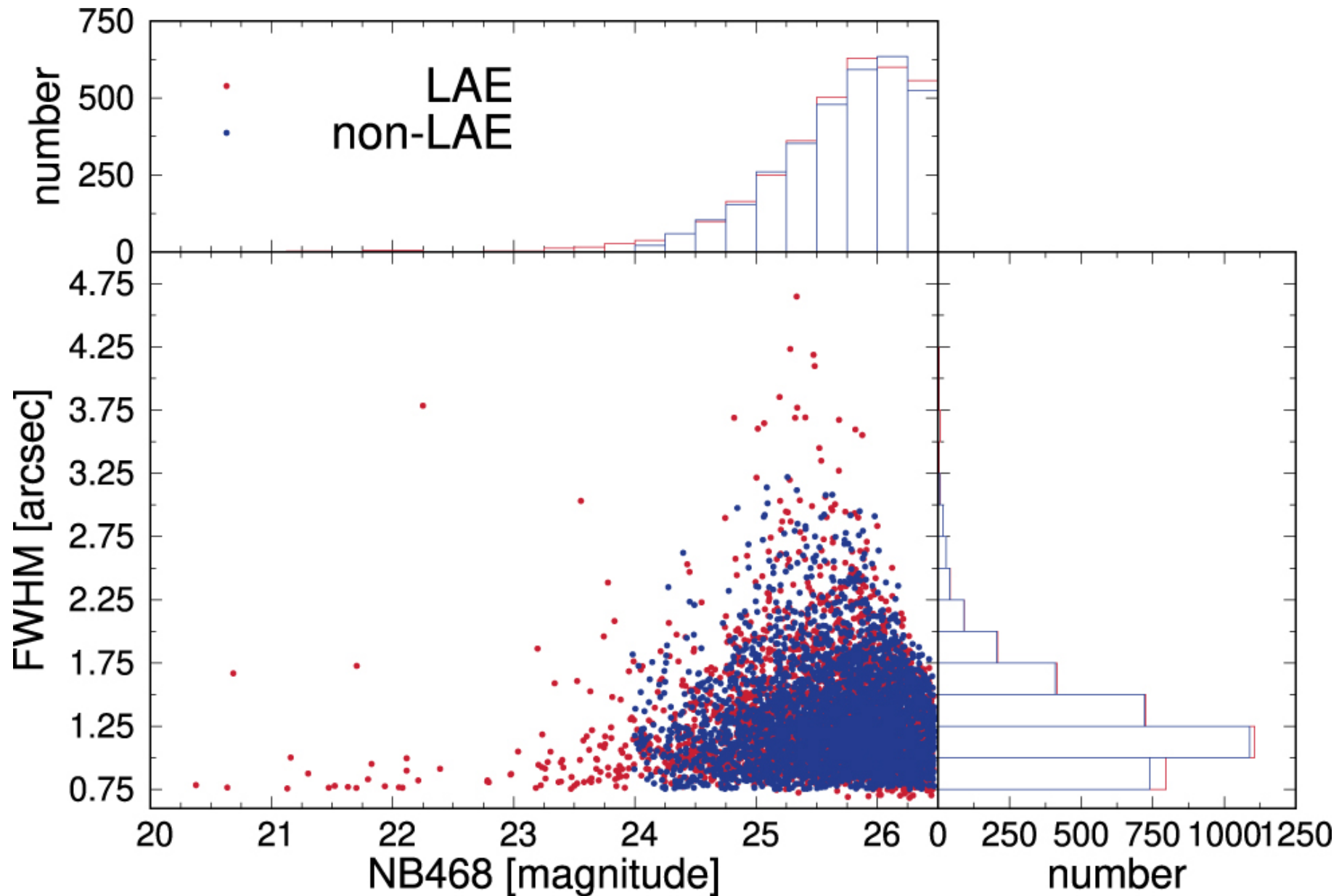
Figure 5. from Satoshi Kikuta et al 2023 Astrophys. J. 947 doi:10.3847/1538-4357/acbf30 https://dx.doi.org/10.3847/1538-4357/acbf30 © 2023. The Author(s). Published by the American Astronomical Society.
