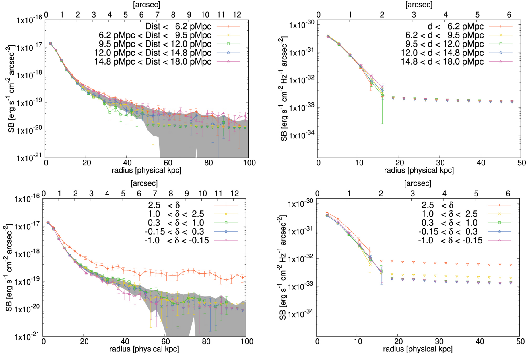
Figure 20. from Satoshi Kikuta et al 2023 Astrophys. J. 947 doi:10.3847/1538-4357/acbf30 https://dx.doi.org/10.3847/1538-4357/acbf30 © 2023. The Author(s). Published by the American Astronomical Society.
