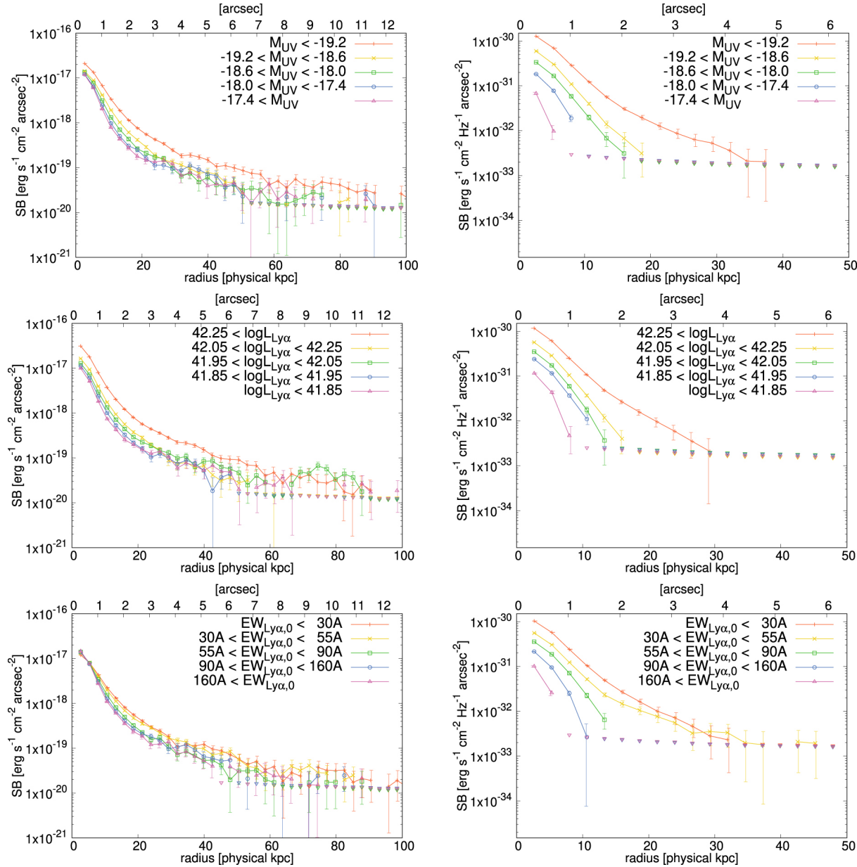
Figure 19. from Satoshi Kikuta et al 2023 Astrophys. J. 947 doi:10.3847/1538-4357/acbf30 https://dx.doi.org/10.3847/1538-4357/acbf30 © 2023. The Author(s). Published by the American Astronomical Society.
