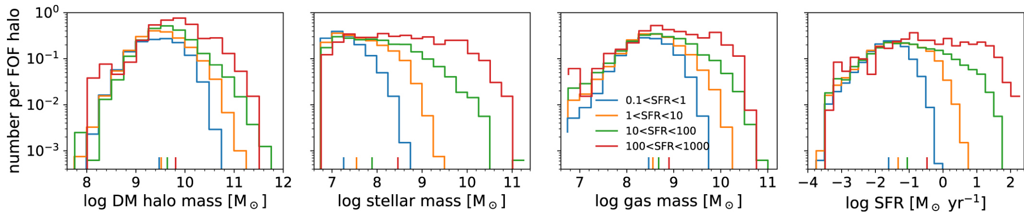
Figure 17. from Satoshi Kikuta et al 2023 Astrophys. J. 947 doi:10.3847/1538-4357/acbf30 https://dx.doi.org/10.3847/1538-4357/acbf30 © 2023. The Author(s). Published by the American Astronomical Society.
