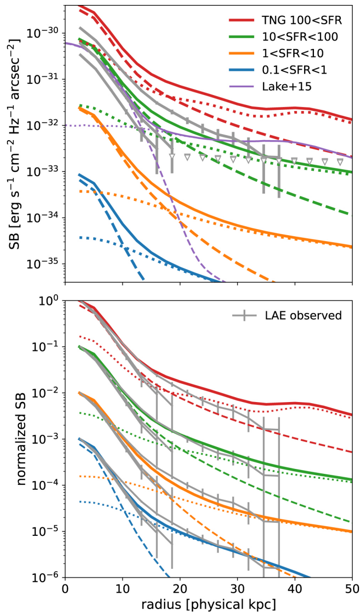
Figure 16. from Satoshi Kikuta et al 2023 Astrophys. J. 947 doi:10.3847/1538-4357/acbf30 https://dx.doi.org/10.3847/1538-4357/acbf30 © 2023. The Author(s). Published by the American Astronomical Society.
