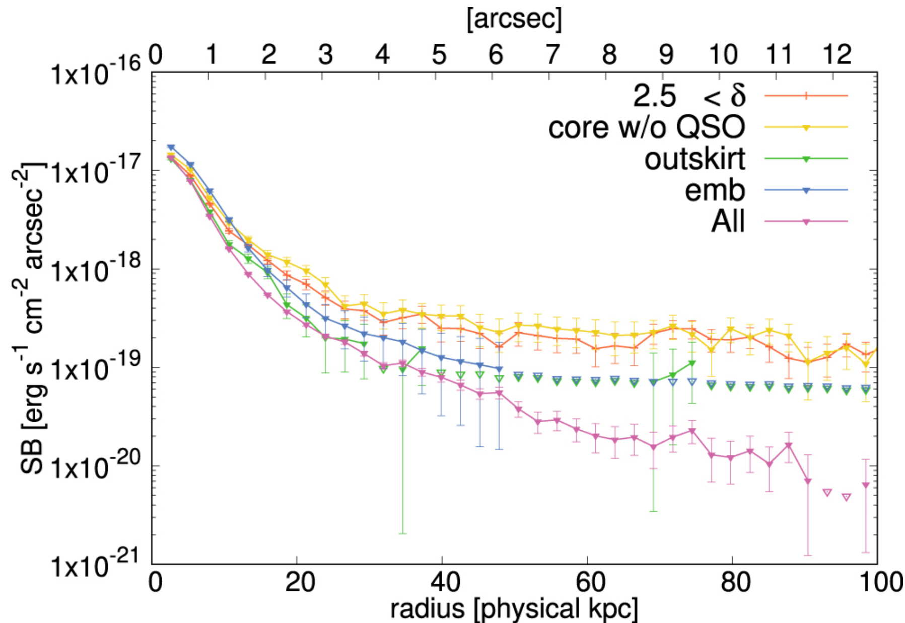
Figure 15. from Satoshi Kikuta et al 2023 Astrophys. J. 947 doi:10.3847/1538-4357/acbf30 https://dx.doi.org/10.3847/1538-4357/acbf30 © 2023. The Author(s). Published by the American Astronomical Society.
