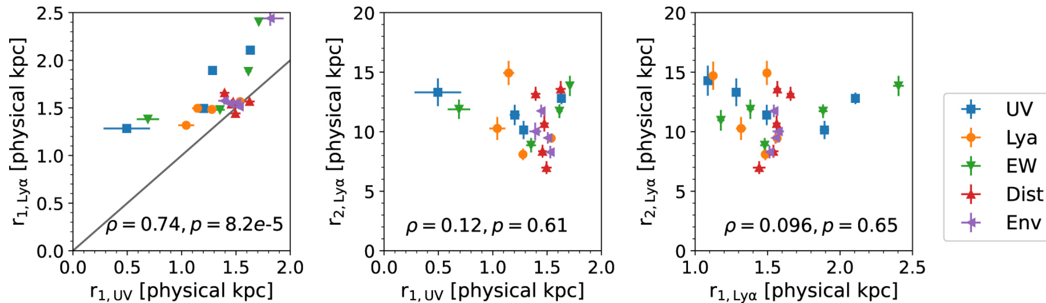
Figure 14. from Satoshi Kikuta et al 2023 Astrophys. J. 947 doi:10.3847/1538-4357/acbf30 https://dx.doi.org/10.3847/1538-4357/acbf30 © 2023. The Author(s). Published by the American Astronomical Society.
