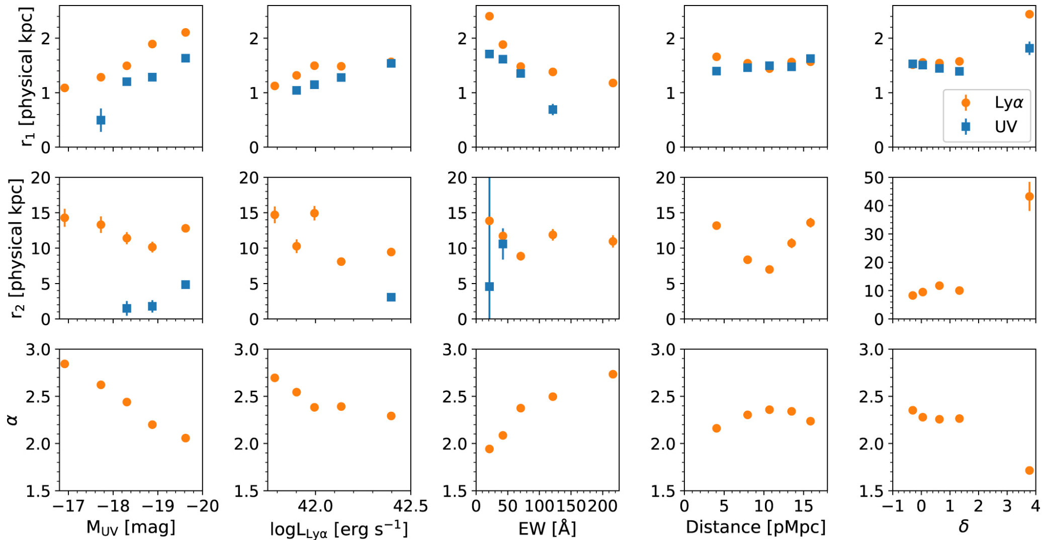
Figure 13. from Satoshi Kikuta et al 2023 Astrophys. J. 947 doi:10.3847/1538-4357/acbf30 https://dx.doi.org/10.3847/1538-4357/acbf30 © 2023. The Author(s). Published by the American Astronomical Society.
