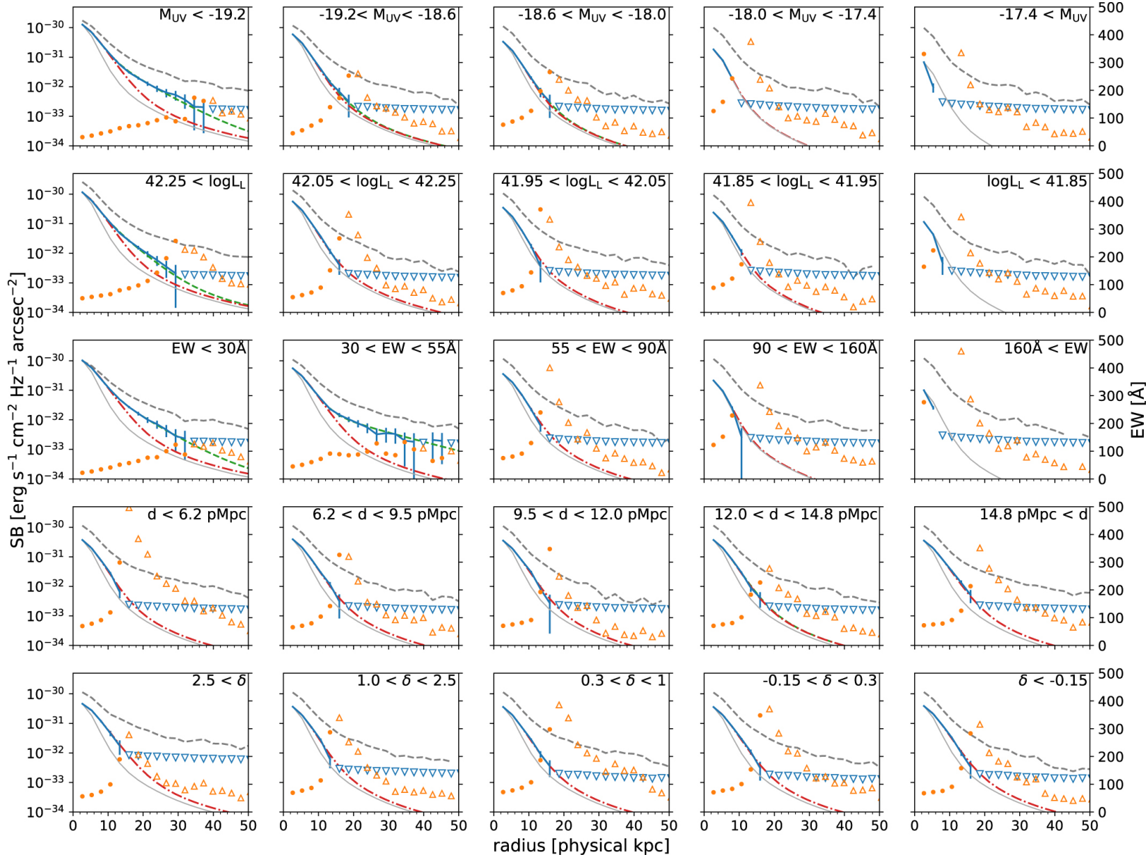
Figure 12. from Satoshi Kikuta et al 2023 Astrophys. J. 947 doi:10.3847/1538-4357/acbf30 https://dx.doi.org/10.3847/1538-4357/acbf30 © 2023. The Author(s). Published by the American Astronomical Society.
