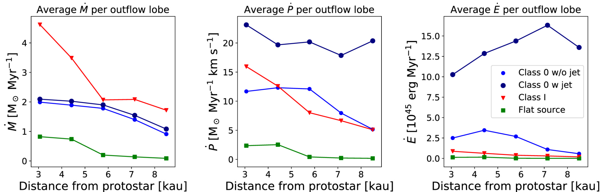
Figure 9. from Cheng-Han Hsieh et al 2023 Astrophys. J. 947 doi:10.3847/1538-4357/acba13 https://dx.doi.org/10.3847/1538-4357/acba13 © 2023. The Author(s). Published by the American Astronomical Society.
