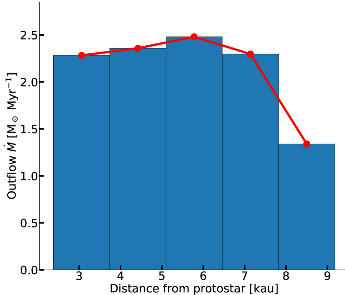
Figure 7. from Cheng-Han Hsieh et al 2023 Astrophys. J. 947 doi:10.3847/1538-4357/acba13 https://dx.doi.org/10.3847/1538-4357/acba13 © 2023. The Author(s). Published by the American Astronomical Society.
