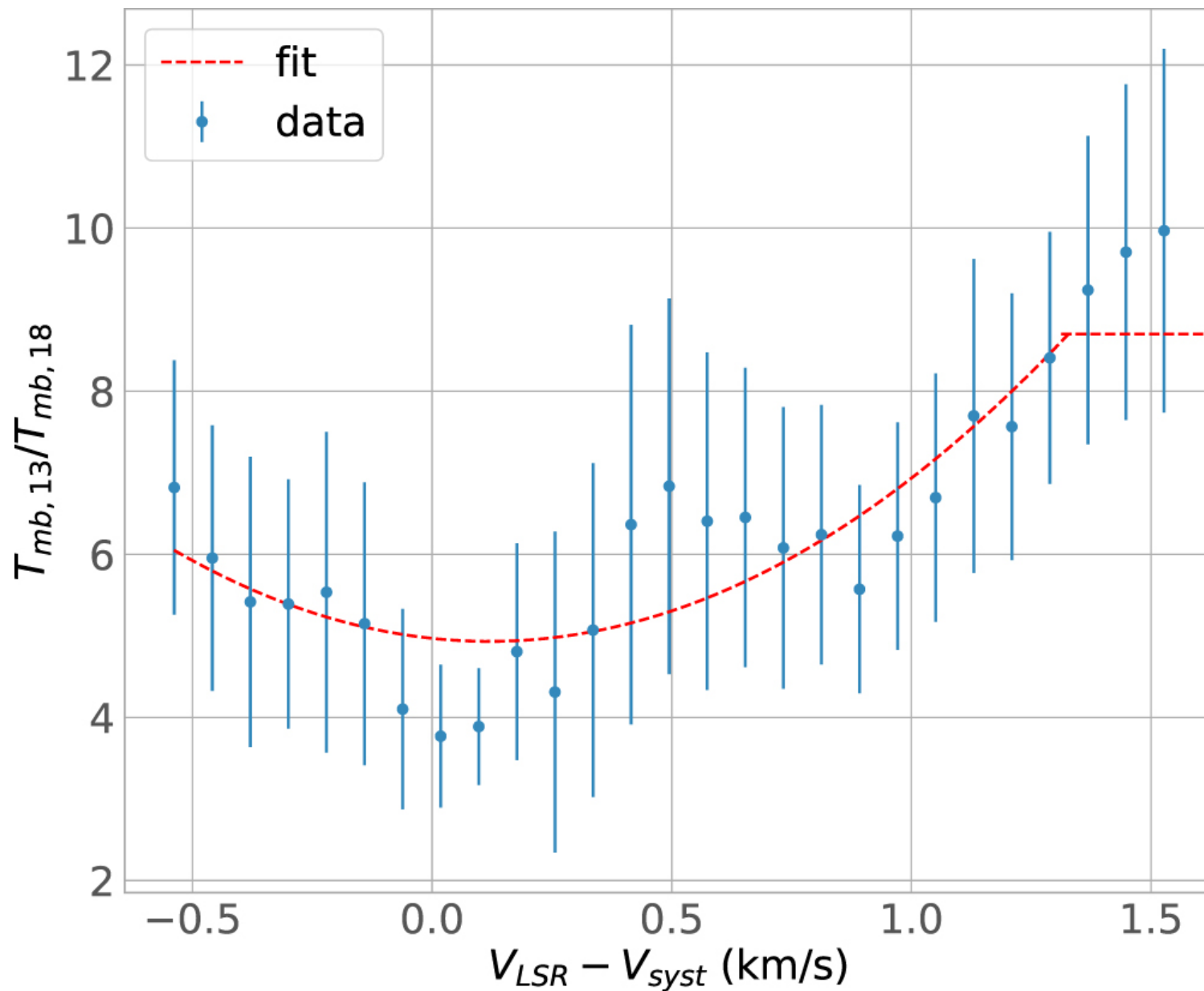
Figure 4. from Cheng-Han Hsieh et al 2023 Astrophys. J. 947 doi:10.3847/1538-4357/acba13 https://dx.doi.org/10.3847/1538-4357/acba13 © 2023. The Author(s). Published by the American Astronomical Society.
