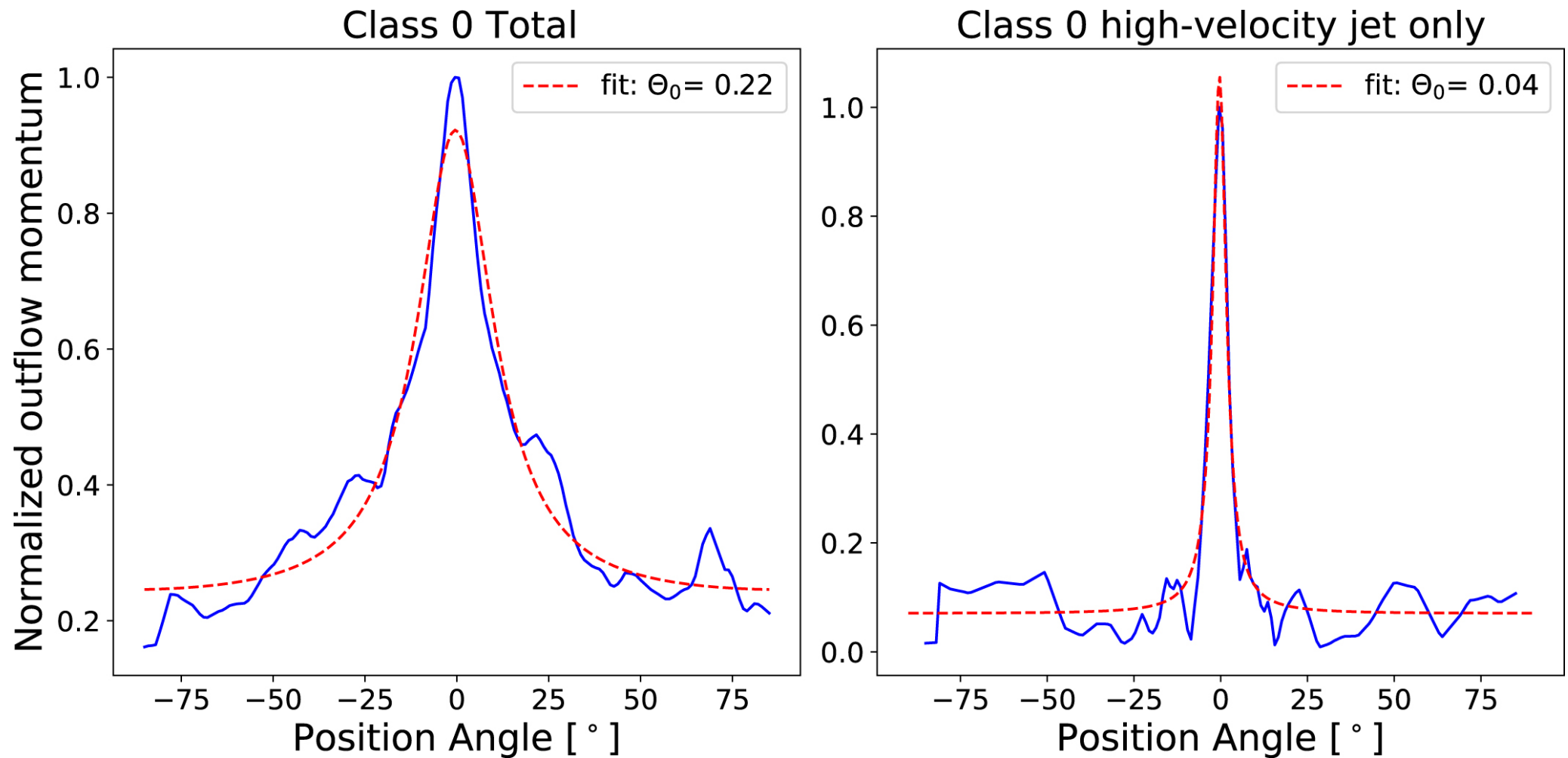
Figure 16. from Cheng-Han Hsieh et al 2023 Astrophys. J. 947 doi:10.3847/1538-4357/acba13 https://dx.doi.org/10.3847/1538-4357/acba13 © 2023. The Author(s). Published by the American Astronomical Society.
