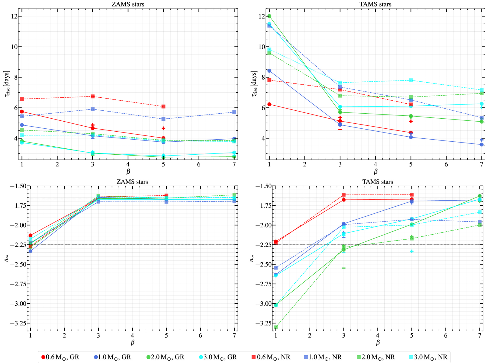
Figure 9. from T. Jankovi and A. Gomboc 2023 Astrophys. J. 946 doi:10.3847/1538-4357/acb8b0 https://dx.doi.org/10.3847/1538-4357/acb8b0 © 2023. The Author(s). Published by the American Astronomical Society.
