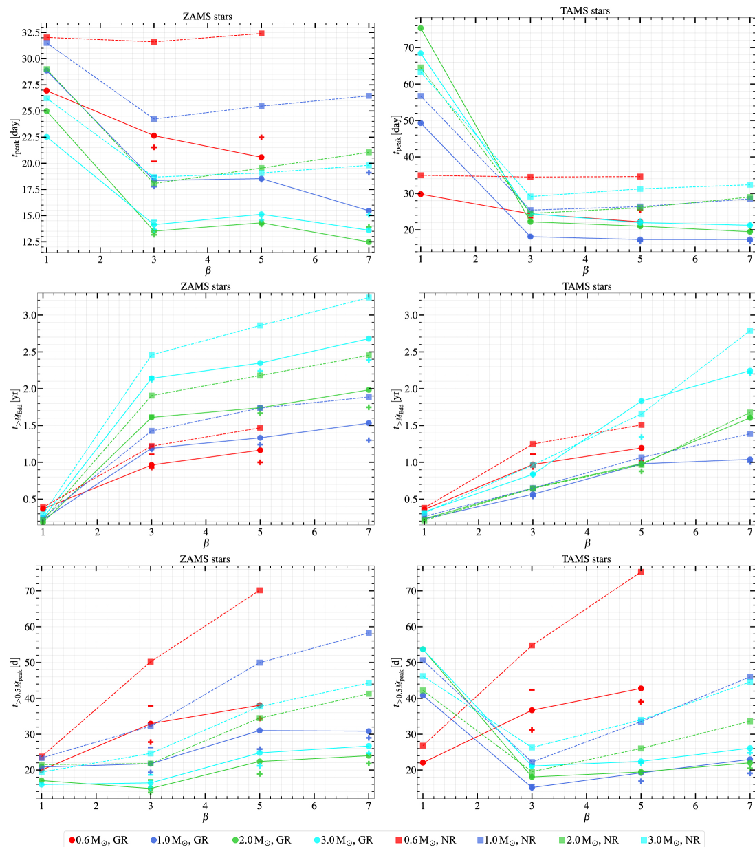
Figure 8. from T. Jankovi and A. Gomboc 2023 Astrophys. J. 946 doi:10.3847/1538-4357/acb8b0 https://dx.doi.org/10.3847/1538-4357/acb8b0 © 2023. The Author(s). Published by the American Astronomical Society.
