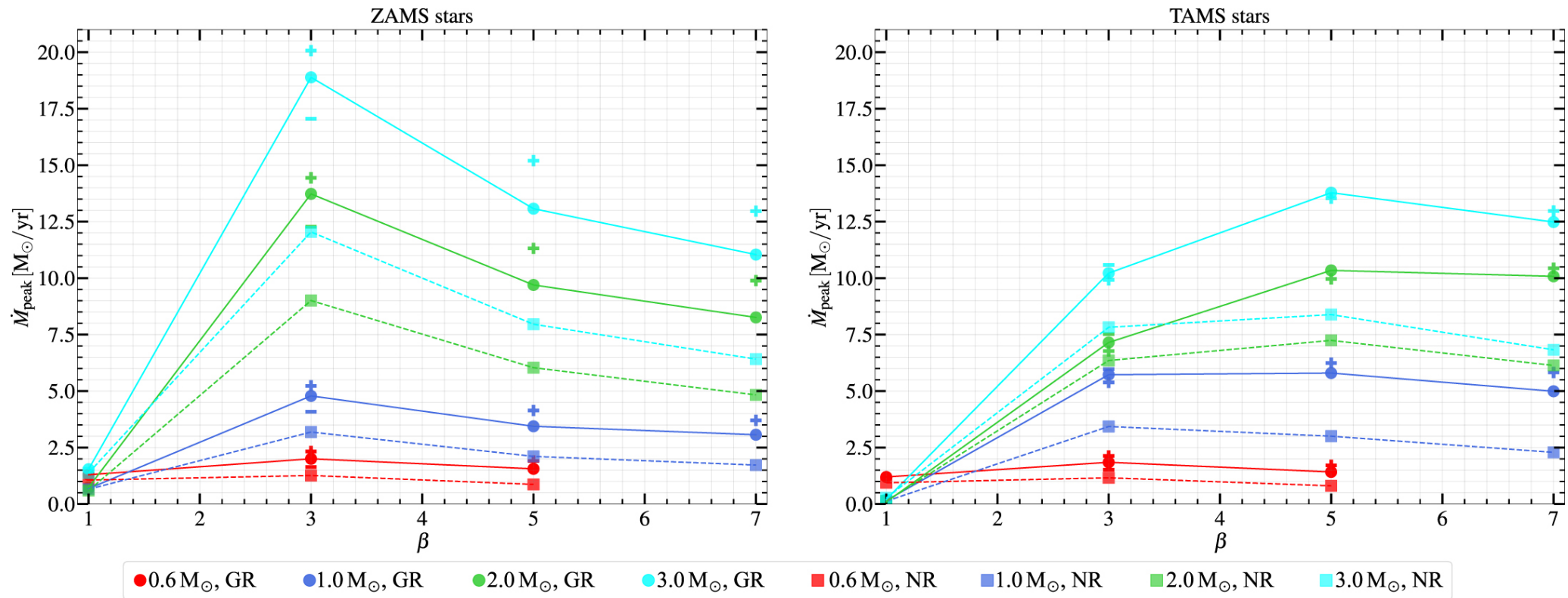
Figure 7. from T. Jankovi and A. Gomboc 2023 Astrophys. J. 946 doi:10.3847/1538-4357/acb8b0 https://dx.doi.org/10.3847/1538-4357/acb8b0 © 2023. The Author(s). Published by the American Astronomical Society.
