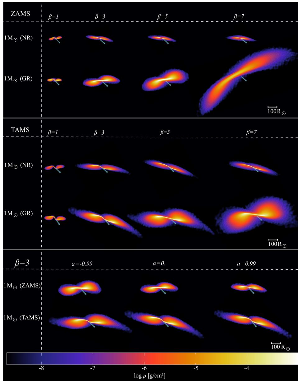
Figure 5. from T. Jankovi and A. Gomboc 2023 Astrophys. J. 946 doi:10.3847/1538-4357/acb8b0 https://dx.doi.org/10.3847/1538-4357/acb8b0 © 2023. The Author(s). Published by the American Astronomical Society.
