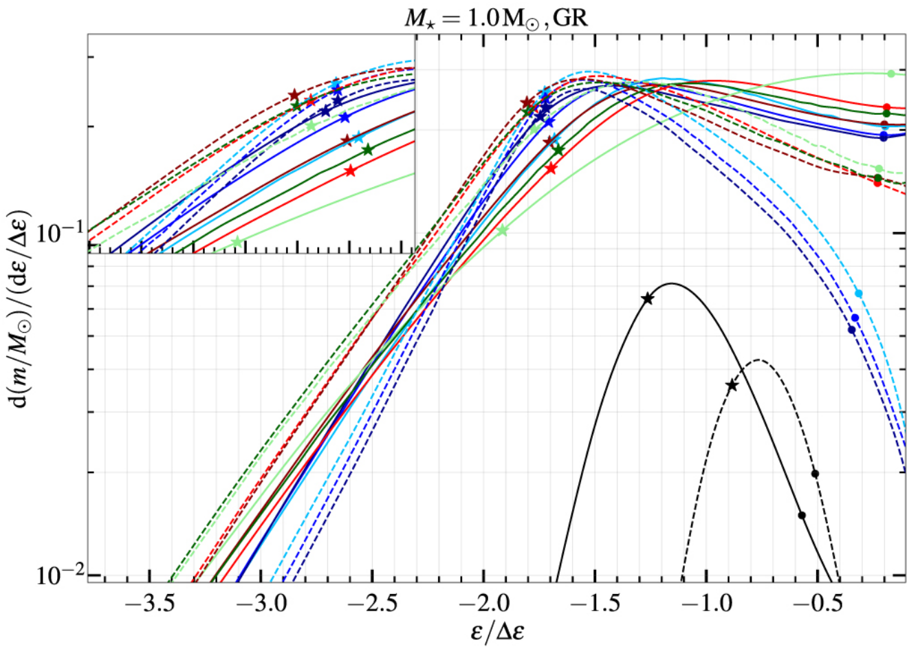
Figure 3. from T. Jankovi and A. Gomboc 2023 Astrophys. J. 946 doi:10.3847/1538-4357/acb8b0 https://dx.doi.org/10.3847/1538-4357/acb8b0 © 2023. The Author(s). Published by the American Astronomical Society.
