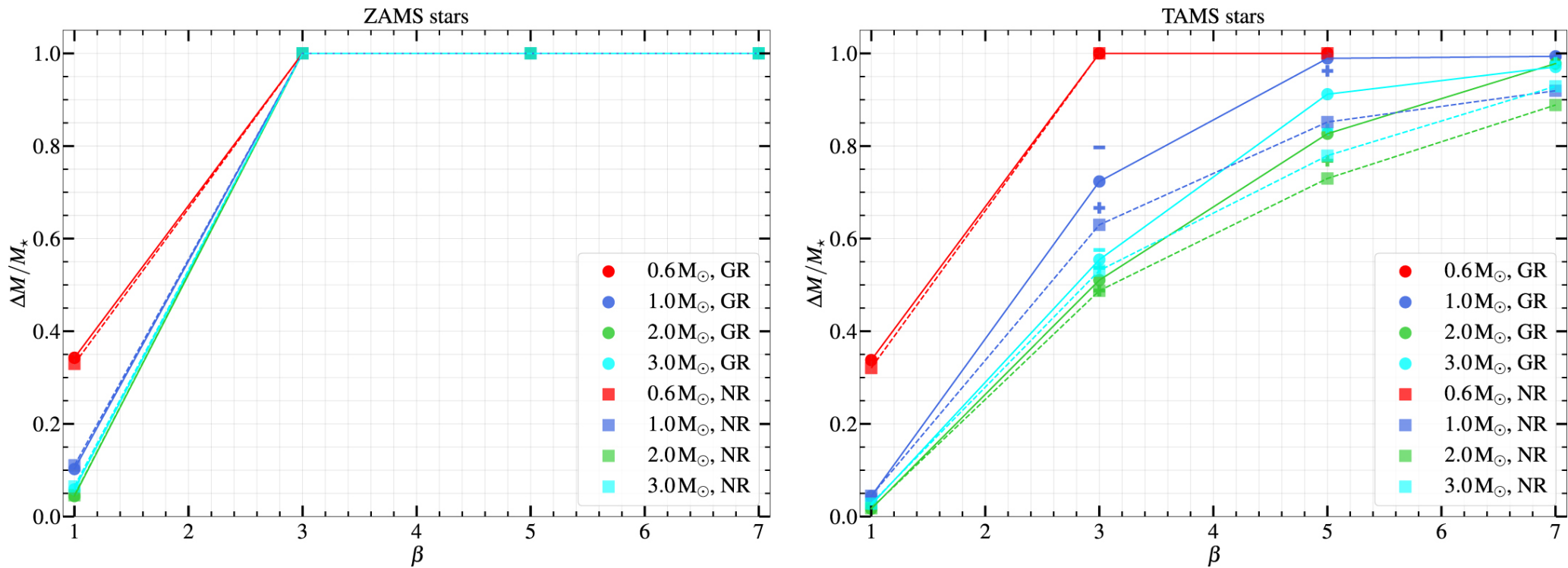
Figure 2. from T. Jankovi and A. Gomboc 2023 Astrophys. J. 946 doi:10.3847/1538-4357/acb8b0 https://dx.doi.org/10.3847/1538-4357/acb8b0 © 2023. The Author(s). Published by the American Astronomical Society.
